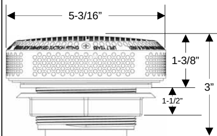
Dimensions shown for both 640-3570V & 640-3580V
