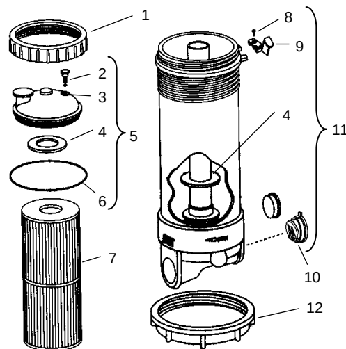
PARTS FOR 17-2540 CHLORINATOR/ BROMINATOR DISPENSER
